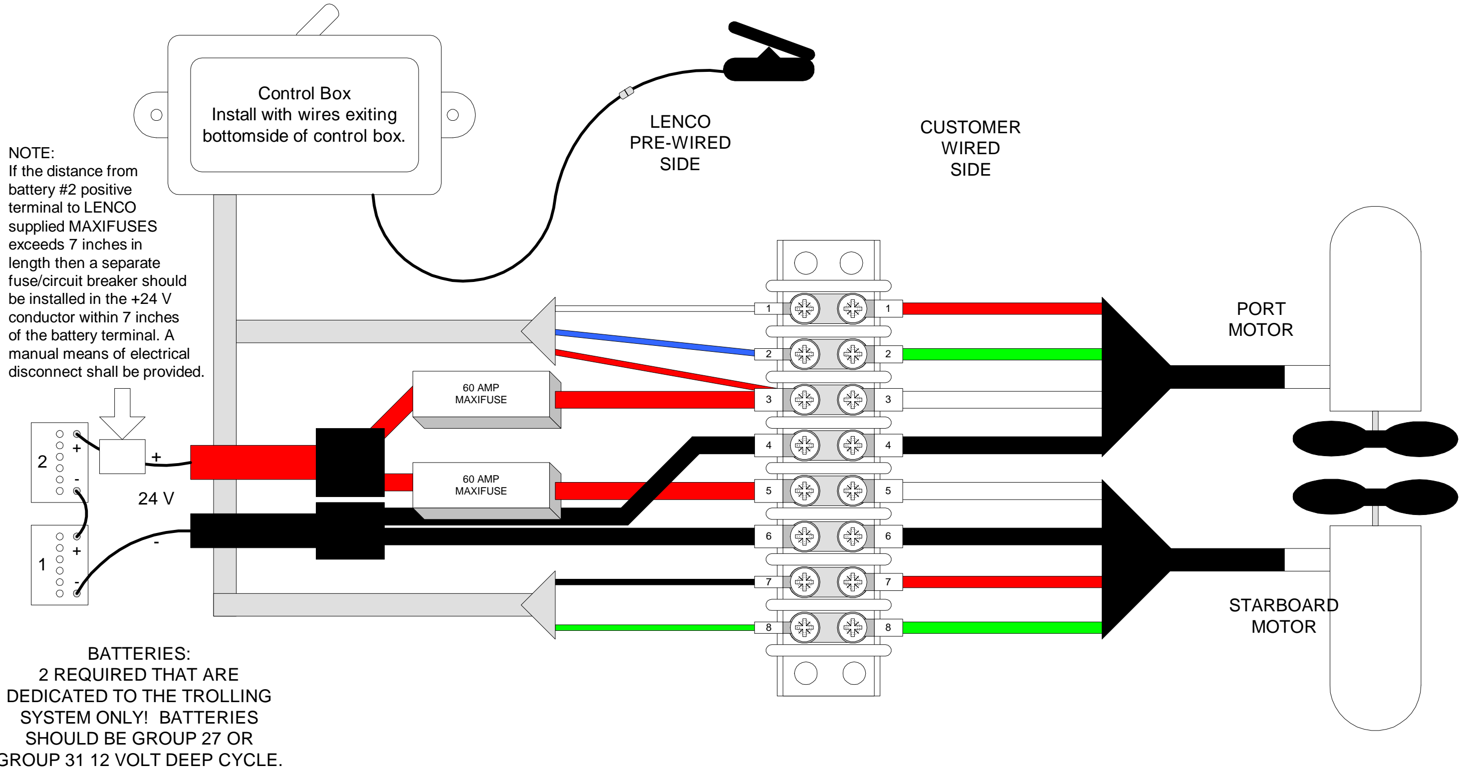
STANDARD 8 POSITION TERMINAL BLOCK USING TWO 4 WIRE MOTORS AND A 5 WIRE CONTROL BOX
